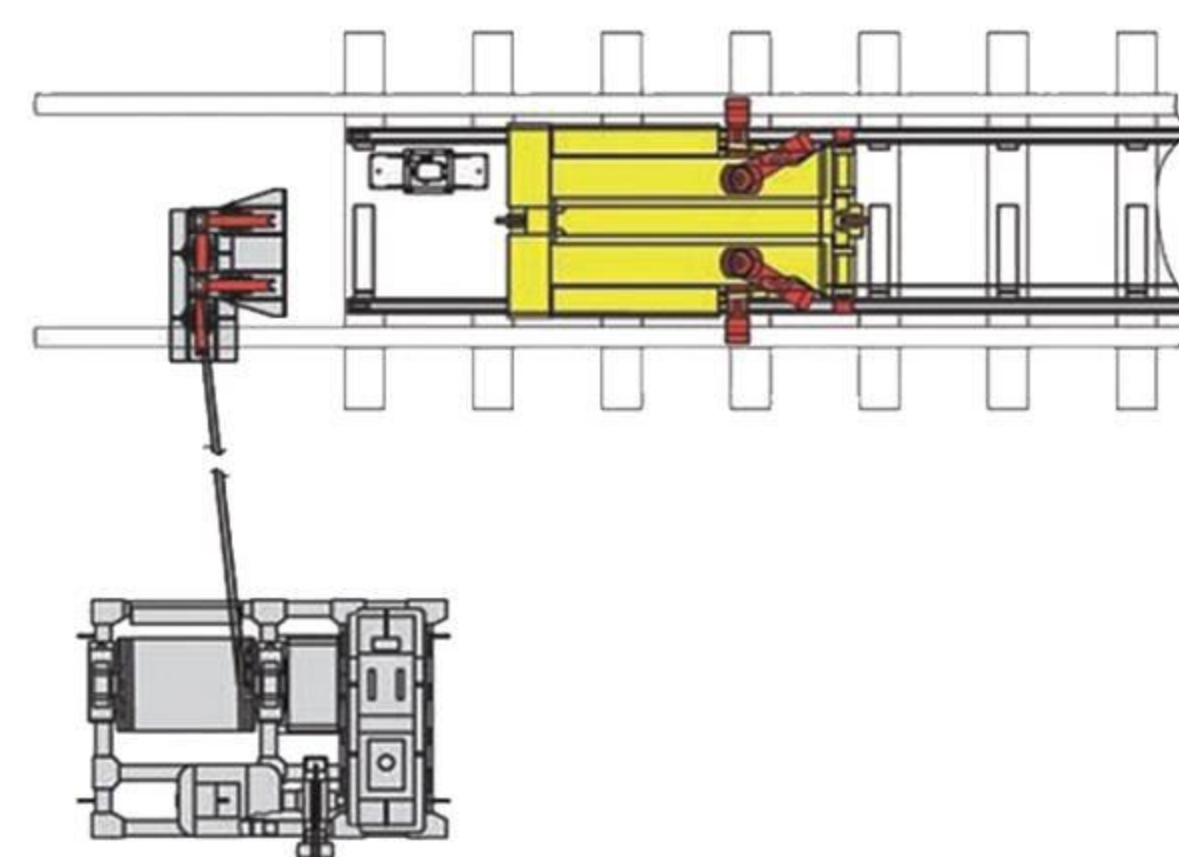
Shunting Facility
