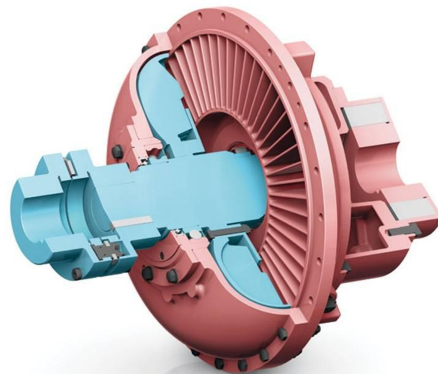
Hydro-coupling
