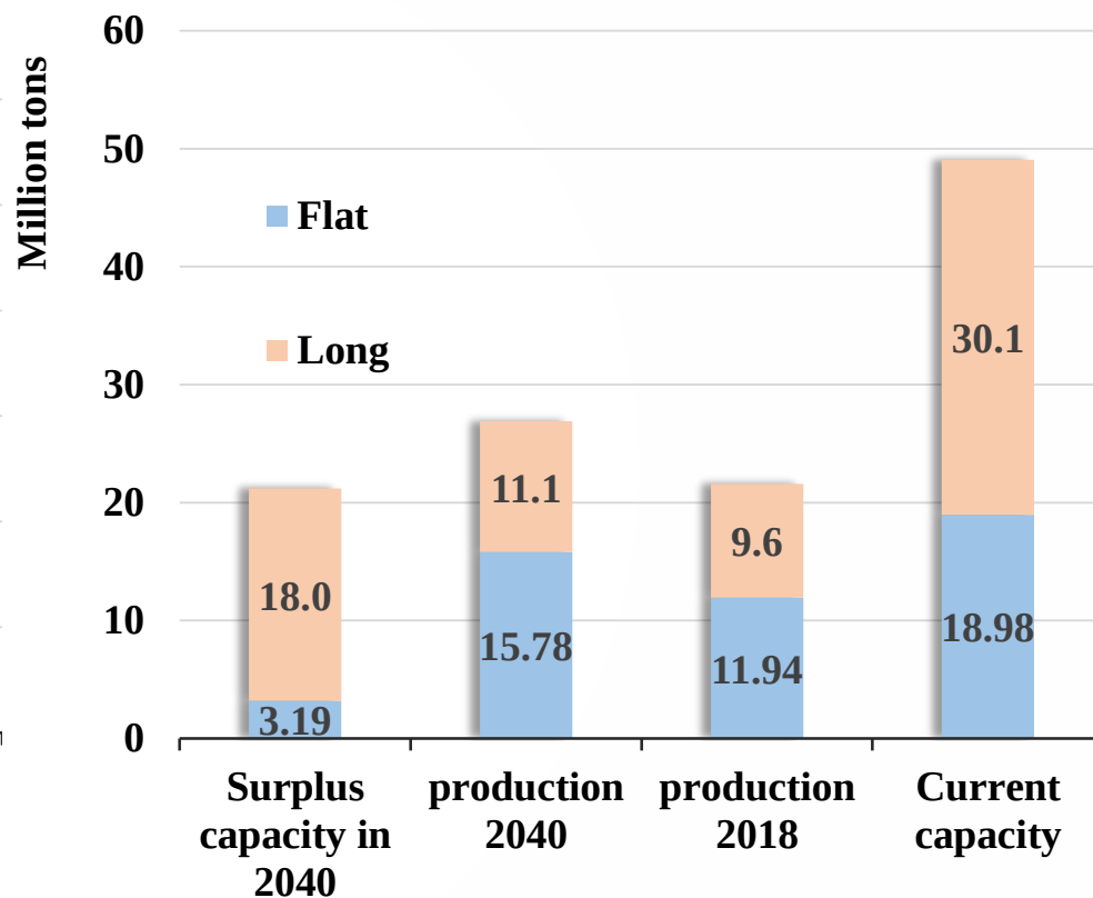
Current and future Iran Finished Steel products
